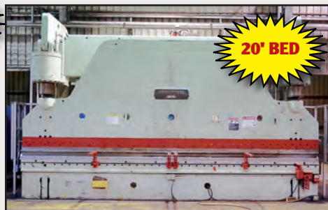
CINCINNATI 500-TON 20' BED, 12' STROKE, WITH MANUAL BACKGAUGE
